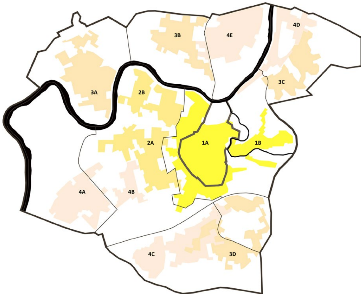
Morphotectonical Ensembles Diagram. The Case of Vilnius Centre
